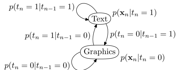
Figure 2. The uni-partite HMM described in Section 2.2. The edges of the graph have been labelled with the corresponding transition probabilities, given in Table 1. Each of the states has an associated emission probability distribution over stroke features, denoted p(\mathbf{x}_n|\cdot) .
