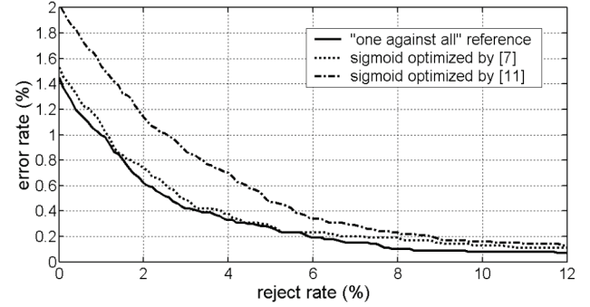
Figure 2. Error-reject tradeoff of "pairwise coupling" on the validation dataset
